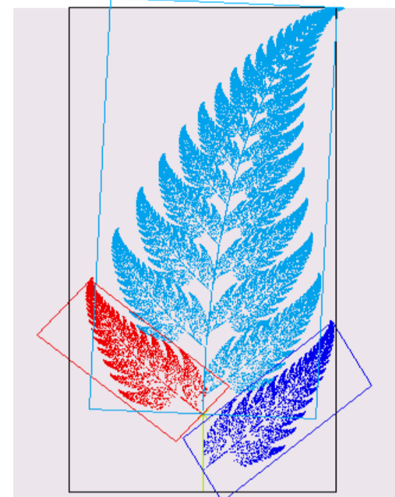
Antônio Miguel de Campos Fractal Fern IFS
